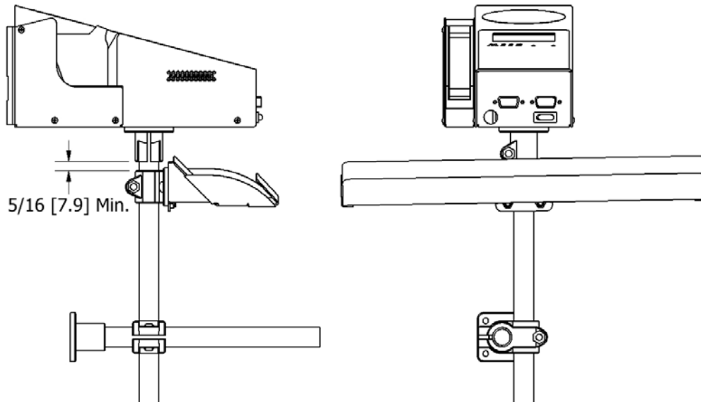
Bulk Ink restraint set-up using the flange clamp
